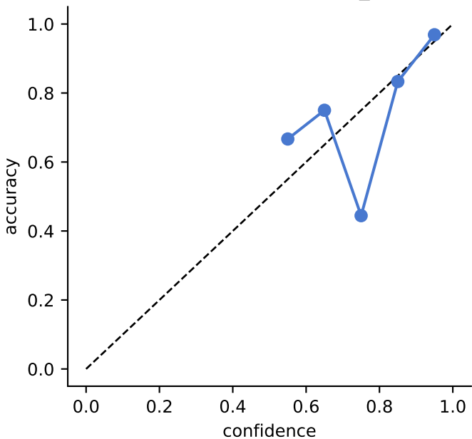
Reliability — ECG5000_BAL
