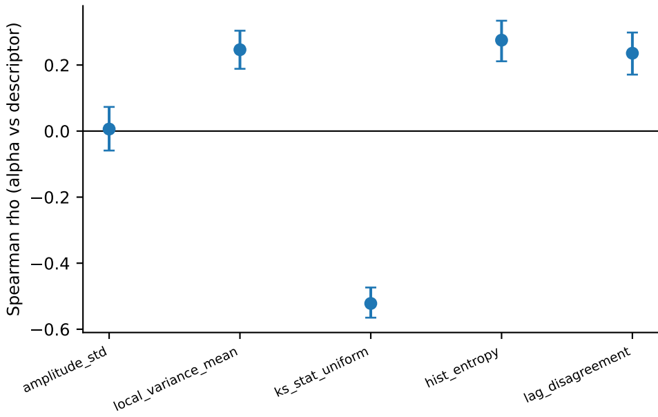
alpha vs independent input descriptors — ECG5000_BAL
