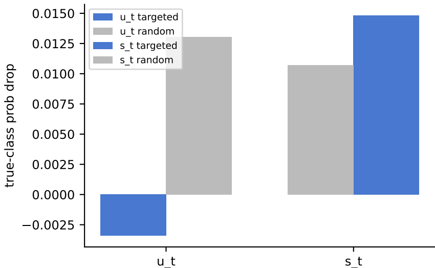
Faithfulness: targeted vs random — ECG5000_BAL
