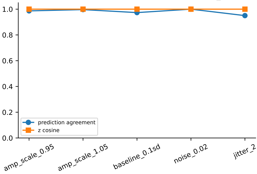
Benign-transformation stability — ECG5000_BAL
