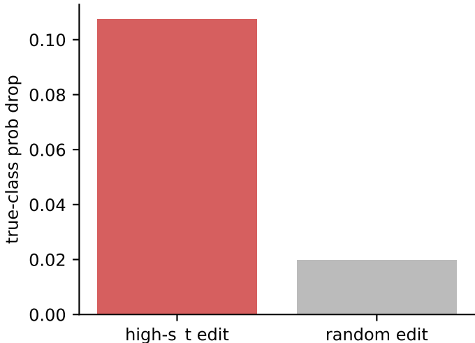
Counterfactual response — ECG5000_BAL
