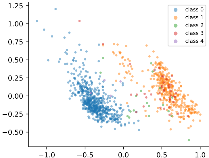
TURS-Lite latent z (pooled) — ECG5000_UNBAL
