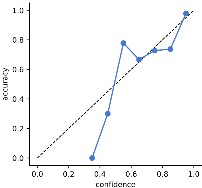
Reliability — ECG5000_UNBAL
