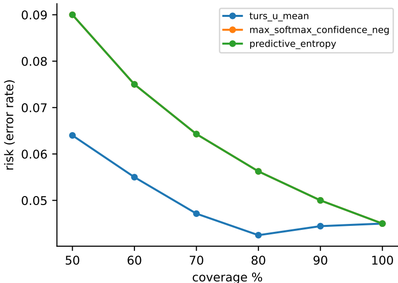
Risk-coverage — ECG5000_UNBAL
