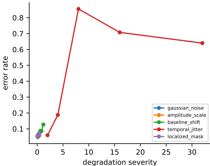
Severity vs error — ECG5000_UNBAL
