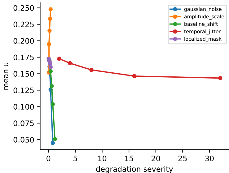
Severity vs u — ECG5000_UNBAL
