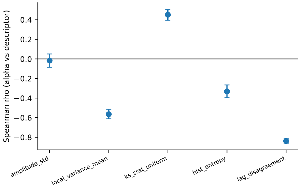
alpha vs independent input descriptors — ECG5000_UNBAL
