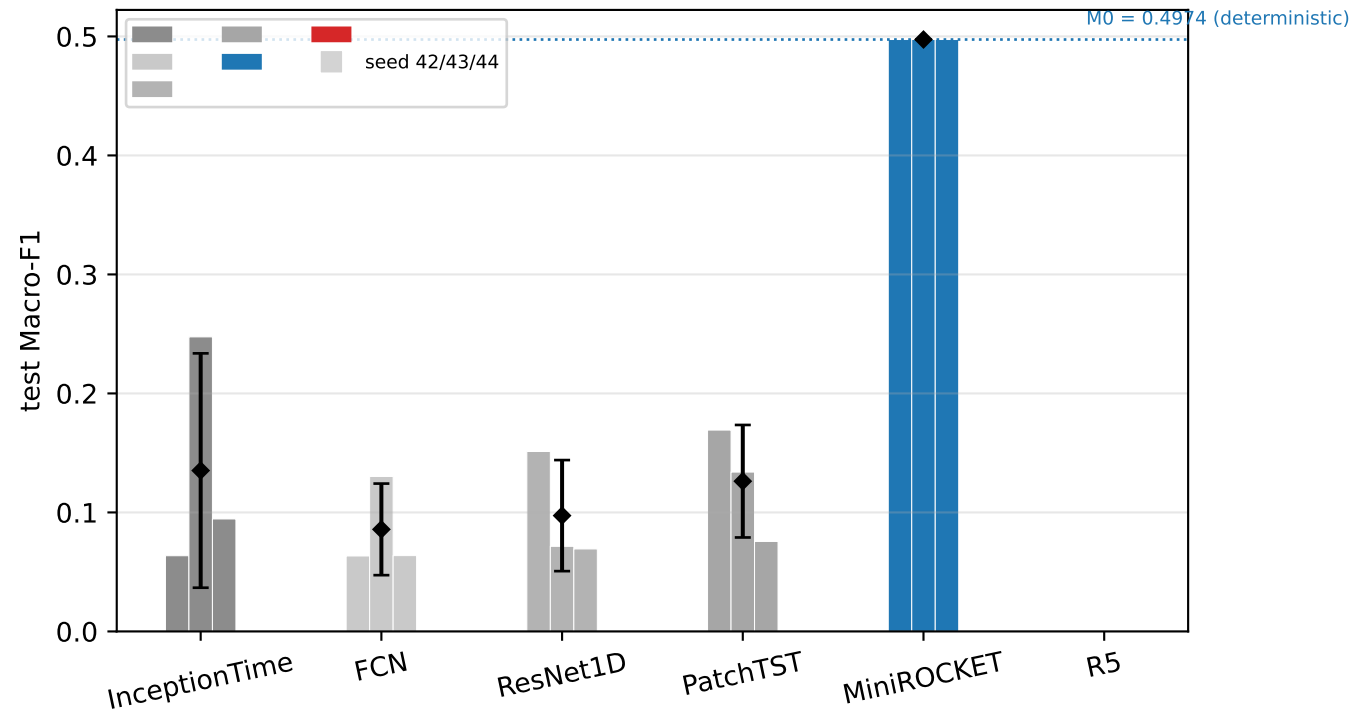
Haptics per-seed test Macro-F1 (diamond = mean \pm SD over seeds)
