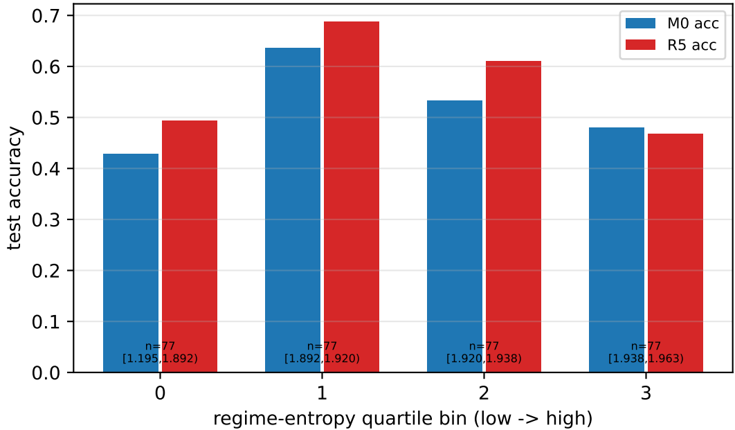
R5 vs M0 accuracy by regime complexity (delta per bin: ['+0.065', '+0.052', '+0.078', '-0.013'])
