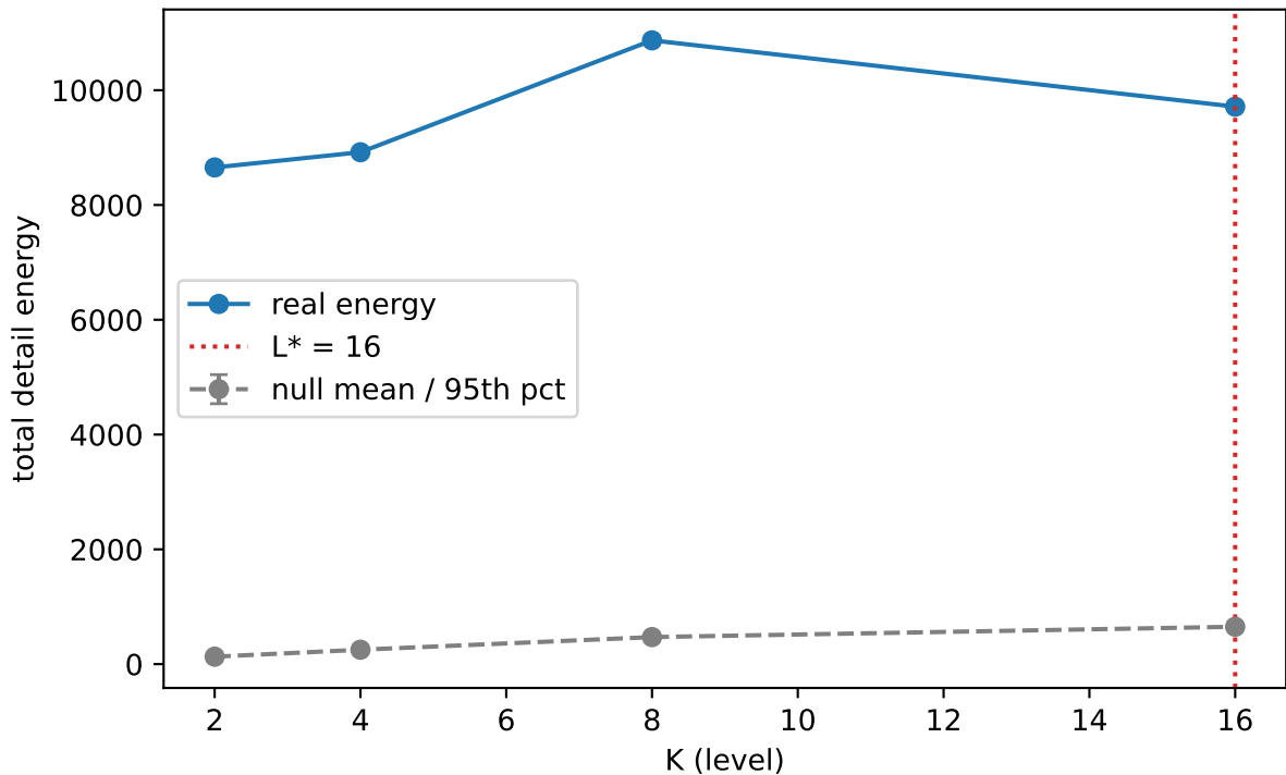
Level energy vs shuffled-regime null
