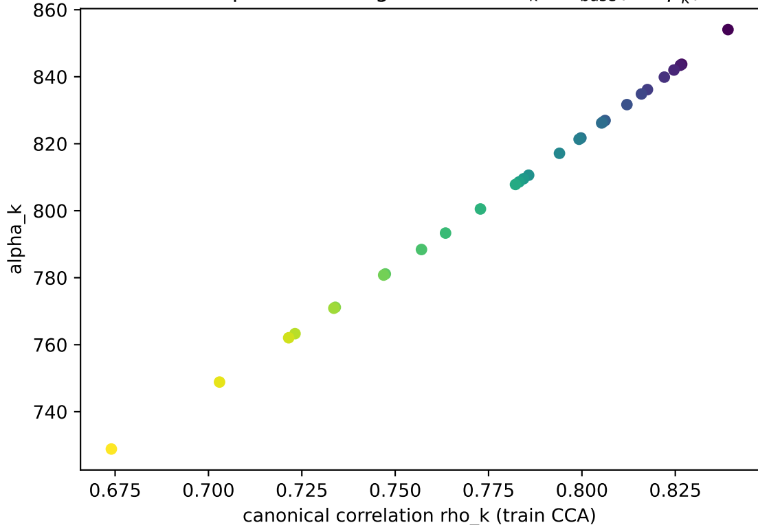
CCA-adaptive shrinkage schedule \alpha_k = \alpha_{base}(1 + \rho_k^2)
