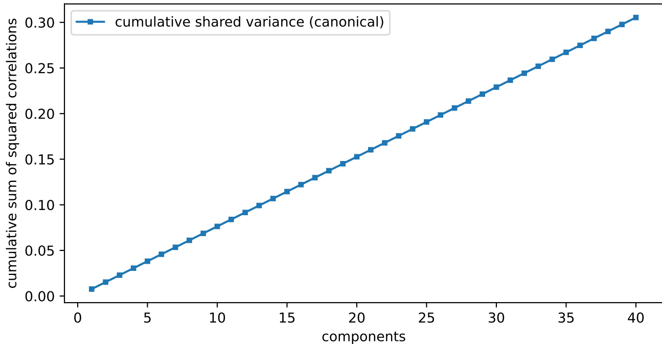
Cumulative shared-correlation diagnostic
