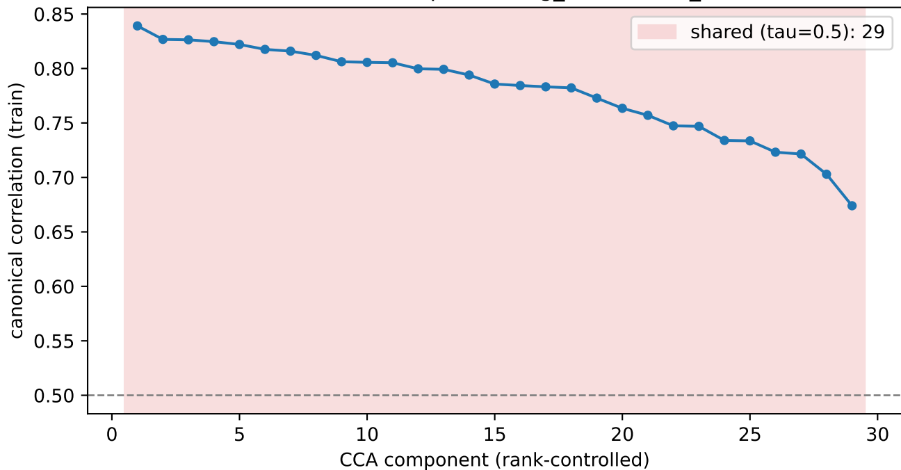
Rank-controlled CCA spectrum (g_rank=29, h_rank=88)
