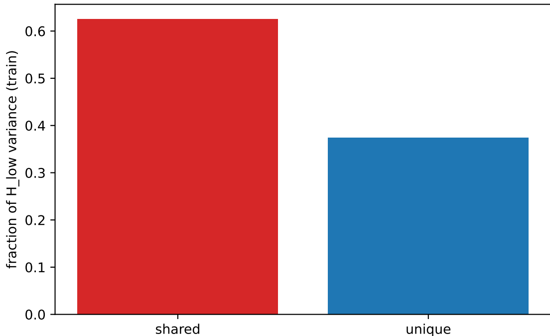
Variance partition (rank-controlled)
