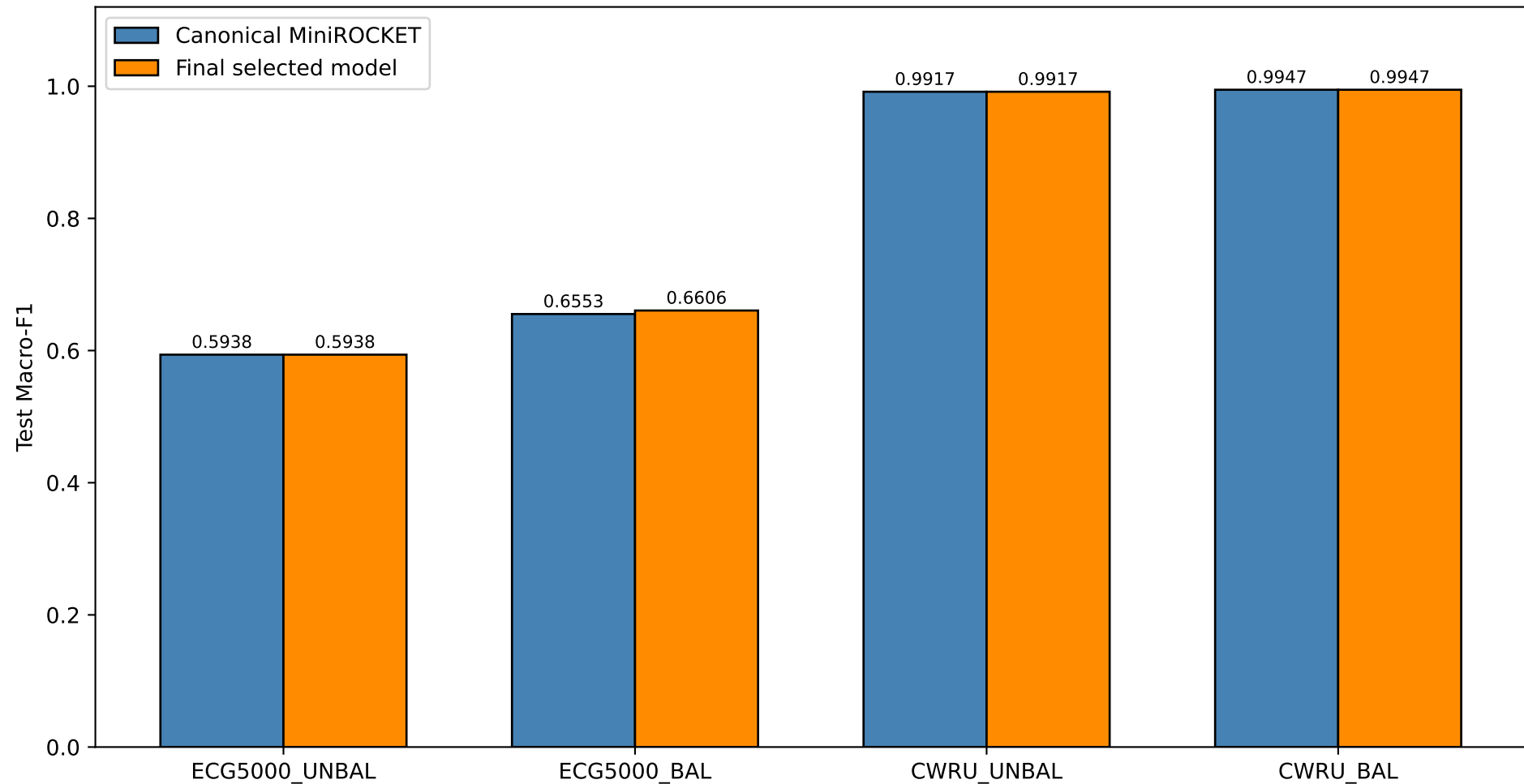
Figure 3: Canonical MiniROCKET vs final gated system (test)
