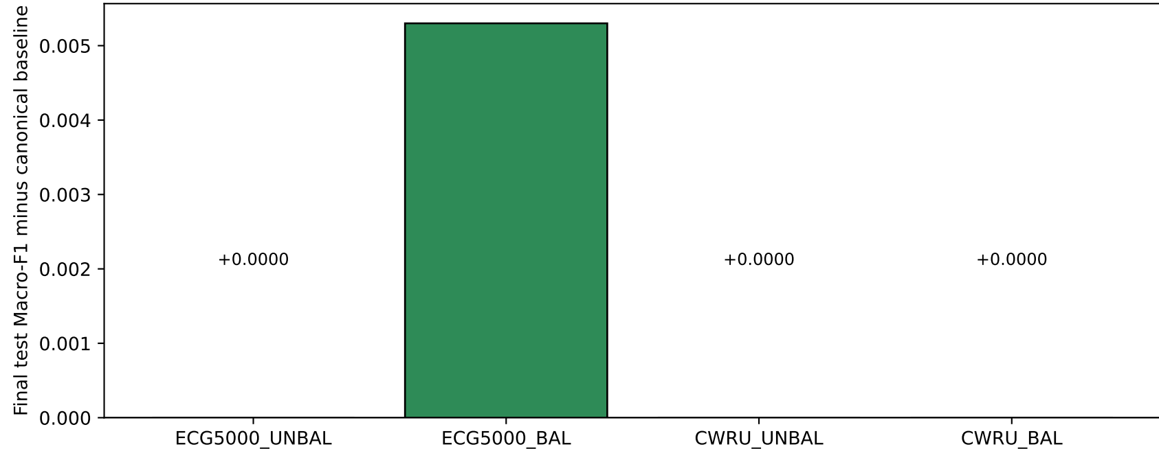
Figure 4: Per-dataset gain/loss of the final gated system
