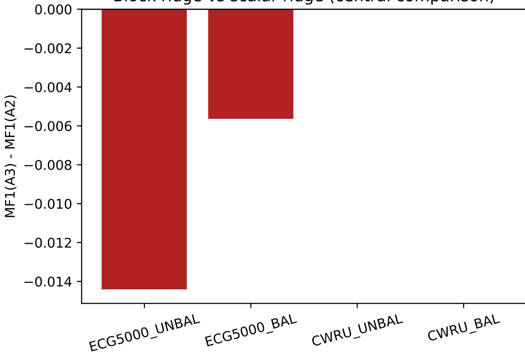
Block ridge vs scalar ridge (central comparison)
