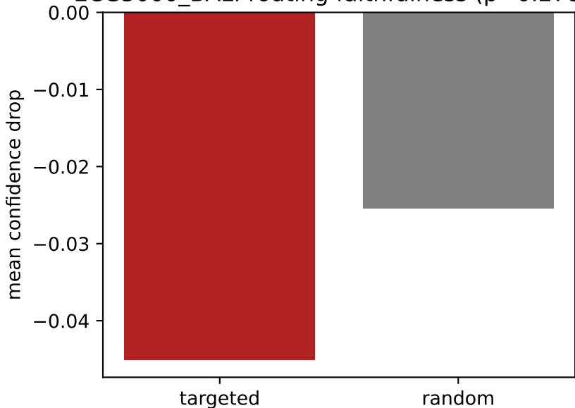
ECG5000_BAL: routing faithfulness ( p=0.2784 )
