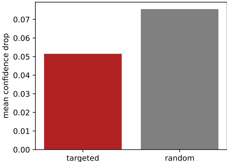
ECG5000_UNBAL: routing faithfulness ( p=0.1524 )
