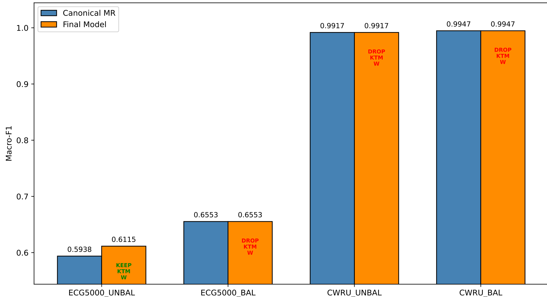
Figure 3: Final Test Performance Canonical MR vs TURS-KTM-AV
