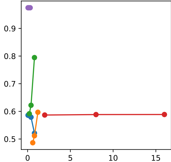
confidence
