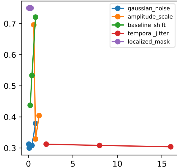
error rate
