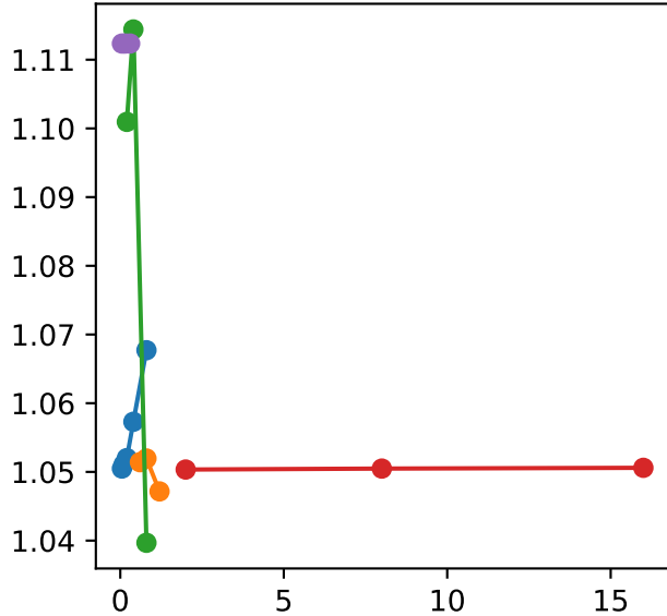
routing entropy
