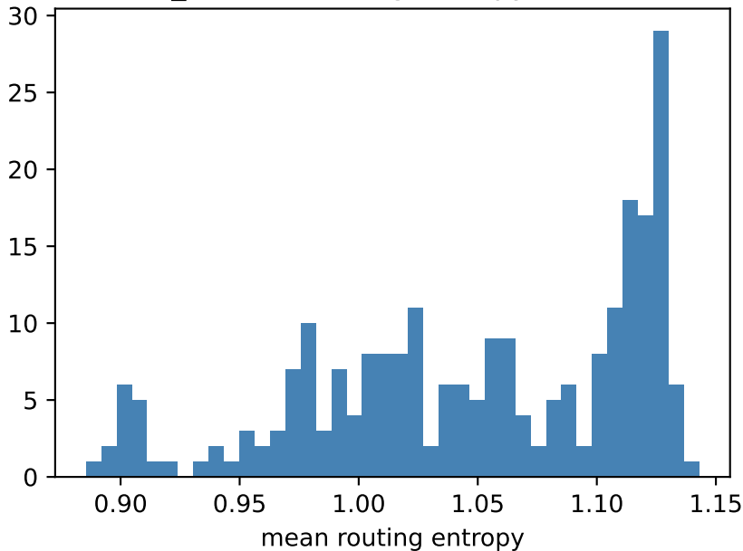
CWRU_UNBAL: routing entropy distribution
