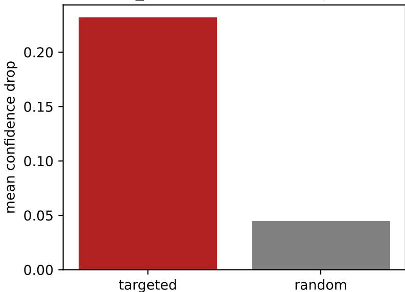
ECG5000_BAL: D4 faithfulness ( p=0.0005 )
