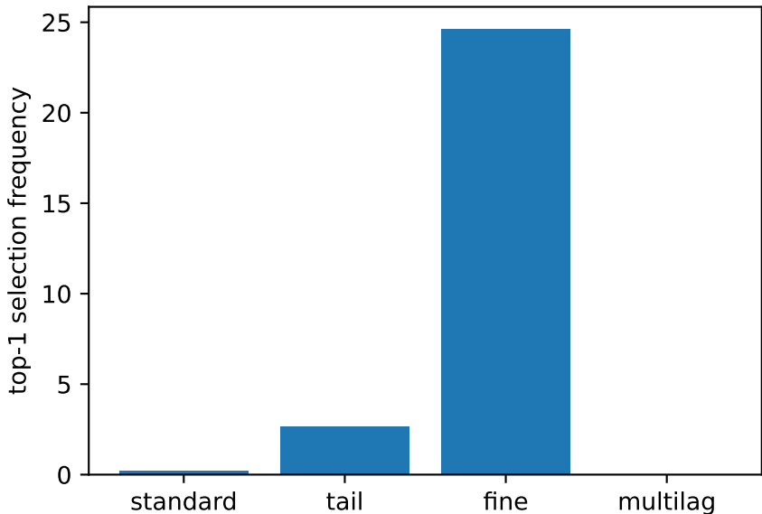
ECG5000_BAL: flavor selection
