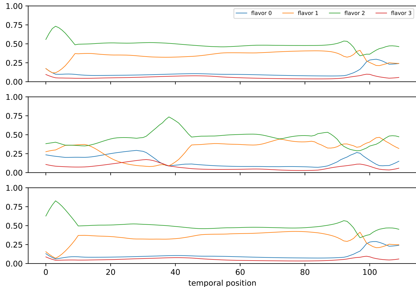
ECG5000_BAL: routing weight timelines (3 test samples)
