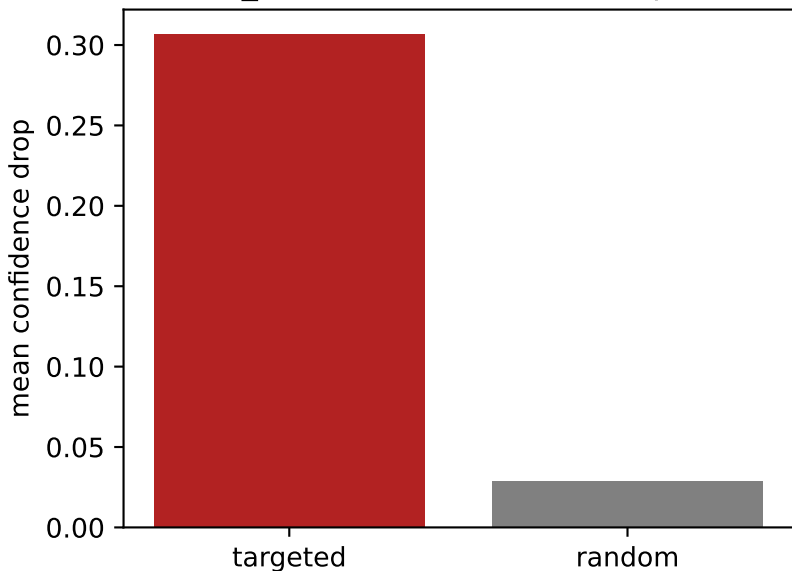
ECG5000_UNBAL: D4 faithfulness ( p=0.0005 )
