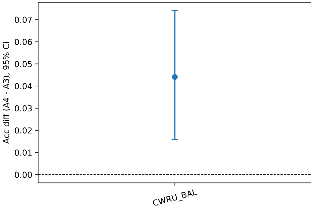
Routing benefit: A4 vs A3 paired accuracy difference
