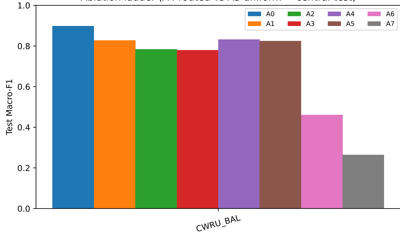
Ablation ladder (A4 routed vs A3 uniform = central test)
