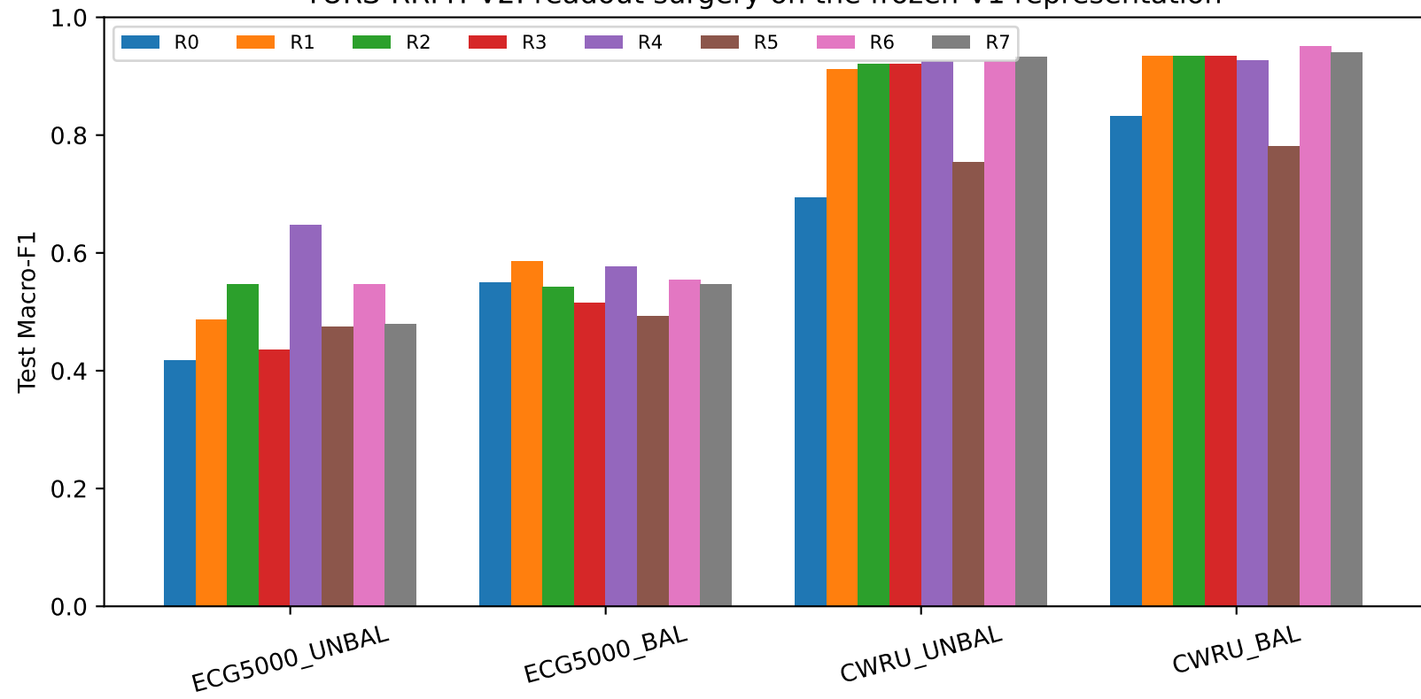
TURS-RRMT-V2: readout surgery on the frozen V1 representation
