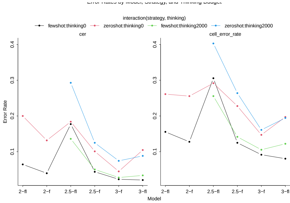
Figure 1: Error rates by model and strategy
