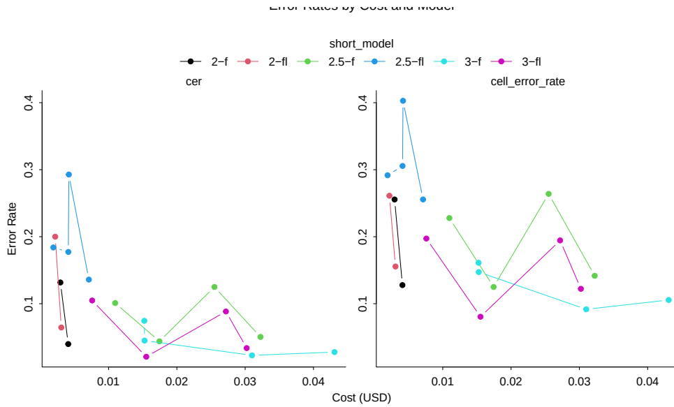
Figure 2: Error rates by cost and model
