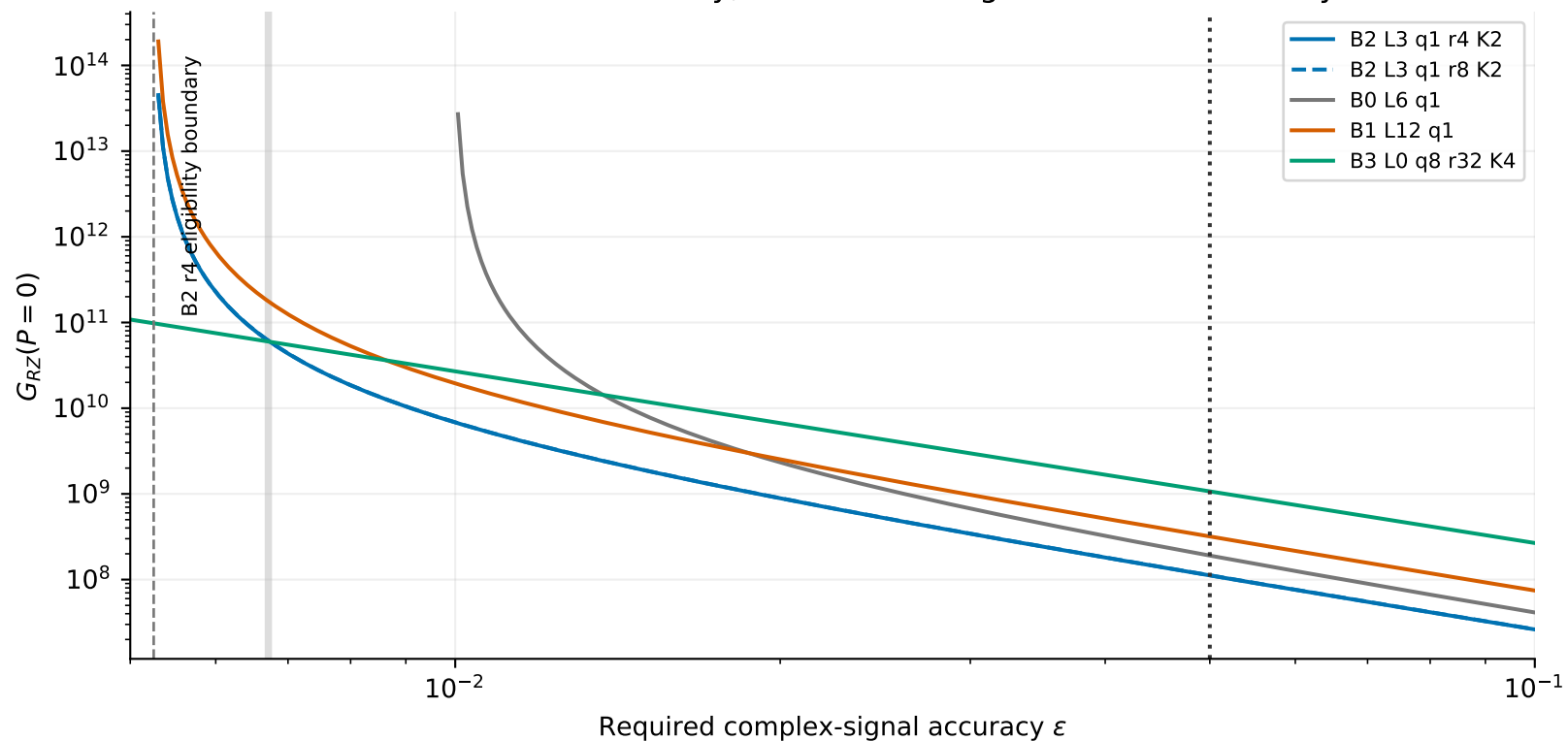
b Posthoc cost sensitivity; dotted line: original transfer accuracy
