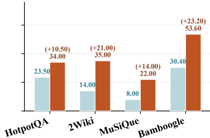
Claude Haiku 4.5
