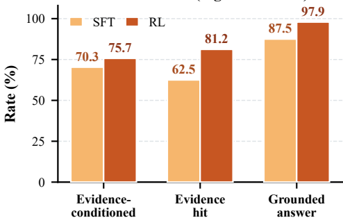
Skill execution (higher is better)
