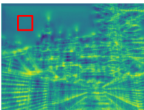
(a)Original Image
