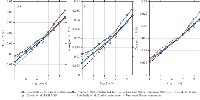
Fig. 8. Low- and moderate-wind MSS comparison for U_{10} = 1\text{--}10 m/s using 20 paired realizations per wind speed. (a) Total MSS. (b) Along-wind MSS. (c) Crosswind MSS. The two simulated groups are compared with observation-derived Cox–Munk, Hu et al., and Guérin slope statistics. The integrated Elfohaily curve is a spectrum-based internal reference rather than a measurement, while the fusion curve denotes the statistical constraint used by the proposed model and is not an independent observation.
