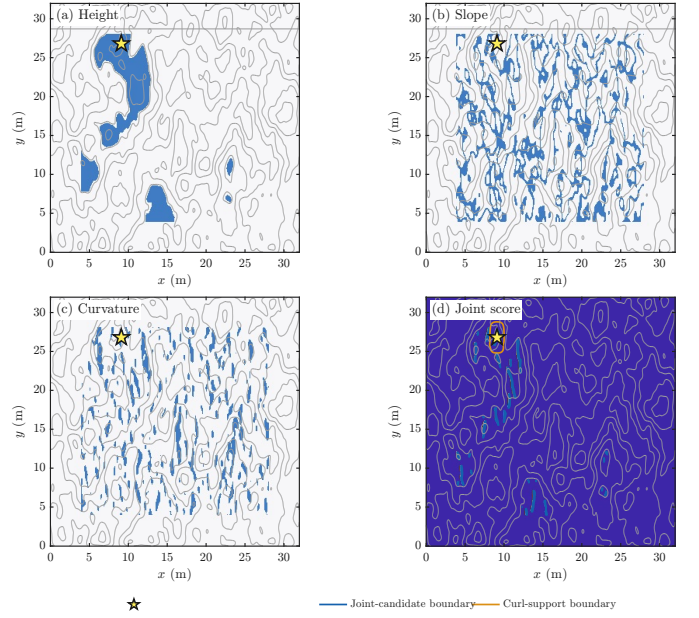
Fig. 3. Breaking-eligible crest selection for U_{10} = 5 m/s, \Omega_c = 0.84 , and H_s = 0.35 m over a 32 \times 32 m 2 surface. The detection uses an elevation quantile of 0.88, a slope-tolerance factor of 0.32, and a negative-curvature quantile of 0.70. (a)–(c) Elevation, near-crest slope, and curvature conditions. (d) Joint candidates, selected crest, and local curling support.
