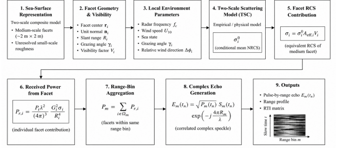
Fig. 7. Processing flow of the facet-based scattering model and statistical radar echo generation.
