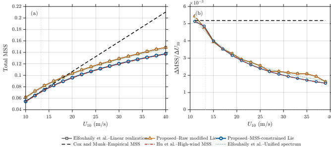
Fig. 9. High-sea-state MSS behavior for U_{10} = 10\text{--}40 m/s using 20 paired realizations per wind speed. (a) Median total MSS of the linear Elfhaily, raw Modified-Lie, and proposed MSS-constrained Lie realizations. The Hu et al. curve is used as the observation-based high-wind MSS reference, the Cox-Munk curve is shown only as a linear empirical extrapolation for comparison, and the integrated Elfhaily curve is a spectrum-based model reference. The vertical marker at U_{10} = 13.3 m/s denotes the transition to the logarithmic Hu high-wind branch. (b) Finite-difference MSS growth rate \Delta \text{MSS} / \Delta U_{10} , illustrating the progressive reduction in wind-speed sensitivity at high sea states.
