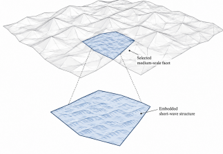
Fig. 6. Scale separation between the resolved medium-scale sea facet and the unresolved short-wave roughness represented statistically.
