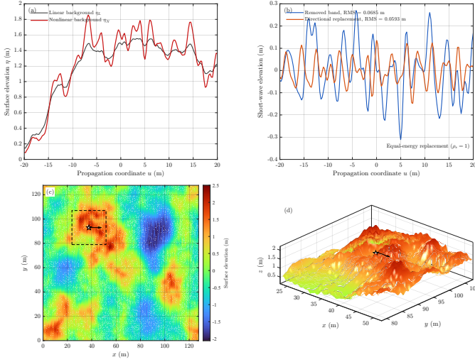
Fig. 2. Nonlinear-background and directional short-wave construction at U_{10} = 10 m/s, \Omega_c = 0.84 , and \phi_w = \psi_s = 0^\circ , over a 128 \times 128 m 2 domain with 0.25 m sampling. (a) Linear and nonlinear propagation-direction profiles. (b) Removed and equal-energy replacement short-wave components for \lambda_s = 1.5 –5.0 m, \sigma_\theta = 8^\circ , and \rho_s = 1 . (c) Combined sea-surface top view. (d) Local 3-D geometry near the selected crest.
