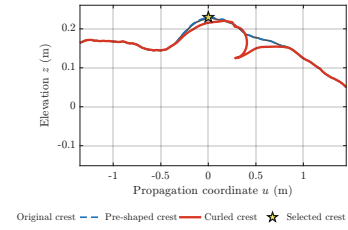
Fig. 5. Propagation-direction section of the selected curling event for U_{10} = 5 m/s and H_s = 0.35 m, showing the original, pre-shaped, and final crest profiles.
