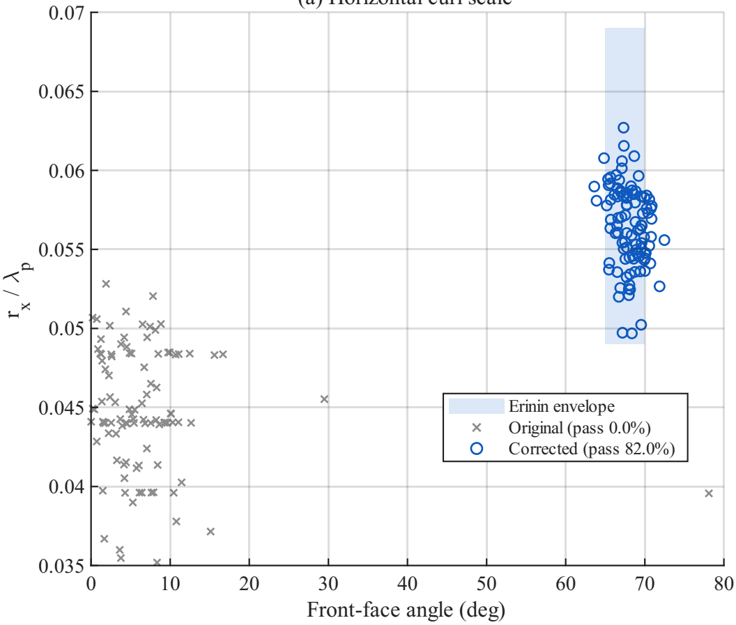
(a) Horizontal curl scale
