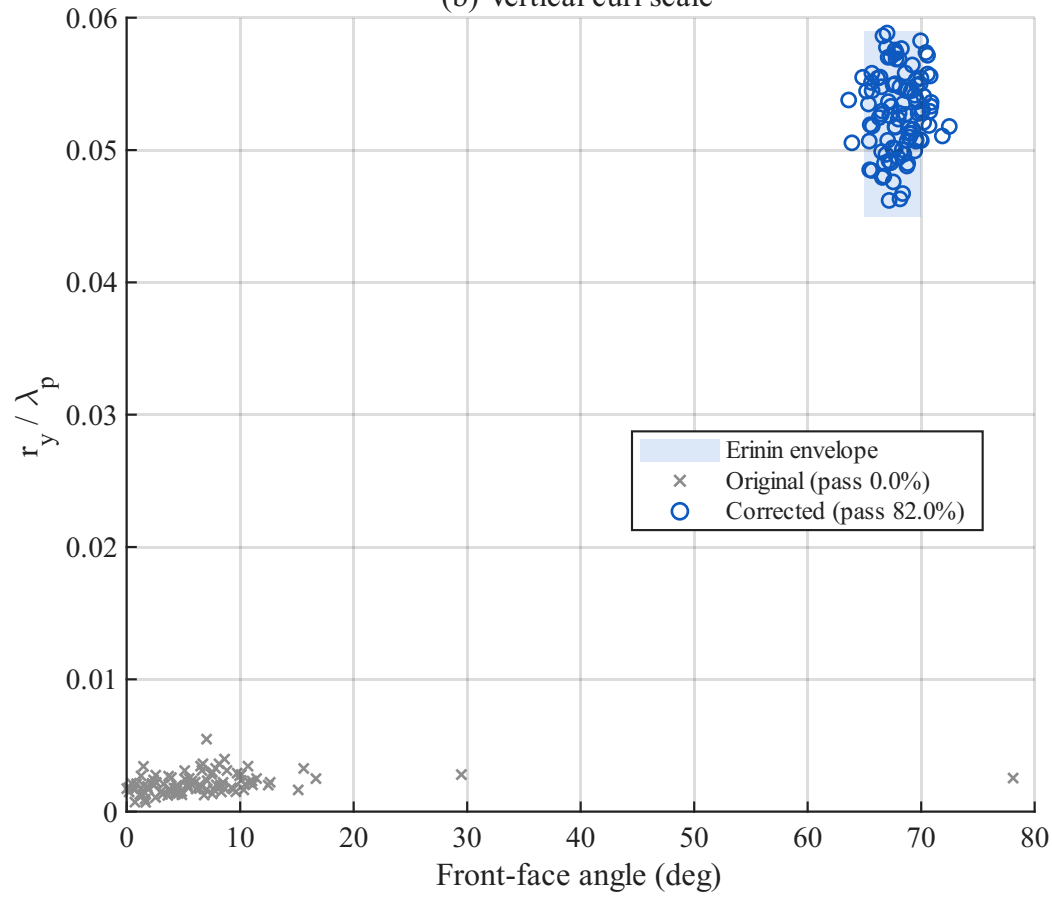
(b) Vertical curl scale
