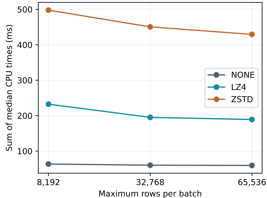
In-memory IPC encode + decode CPU
