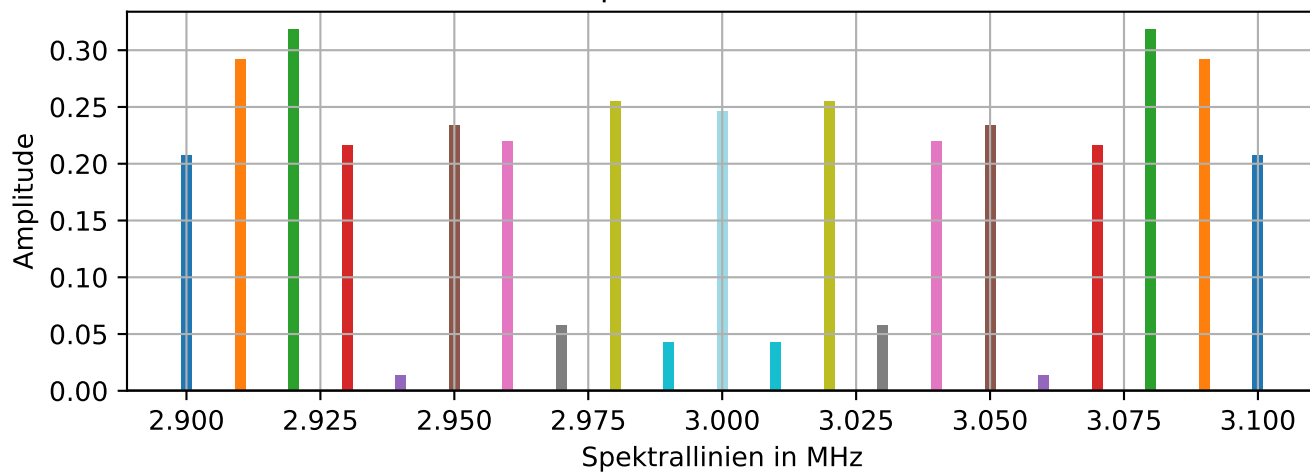
Spektrum m = 10
