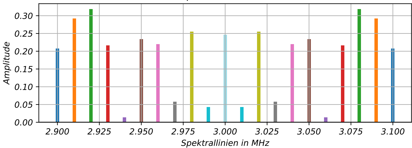
Spektrum m = 10
