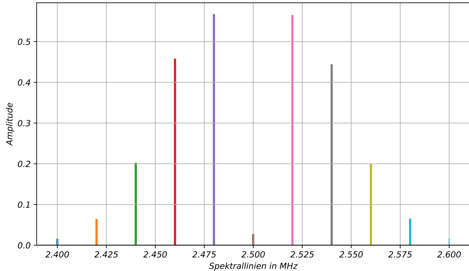
Messspektrum f_1 = 20 \text{ kHz} m = 2.4
