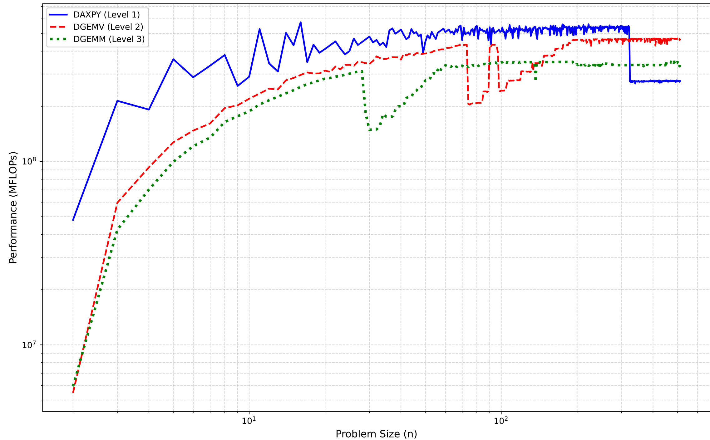
BLAS Performance Comparison (log-log)
