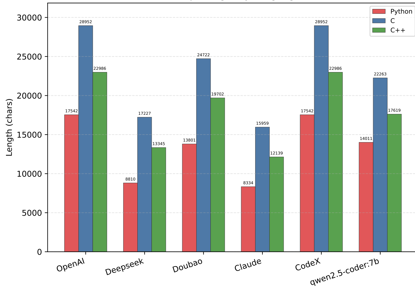
Prompt Length by Language
