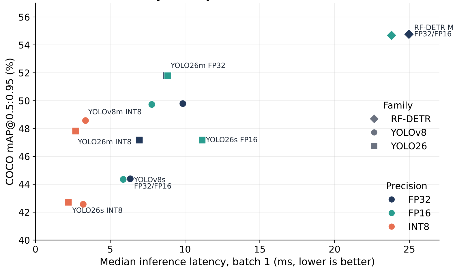
Accuracy-latency trade-off on RTX 3070 Ti
