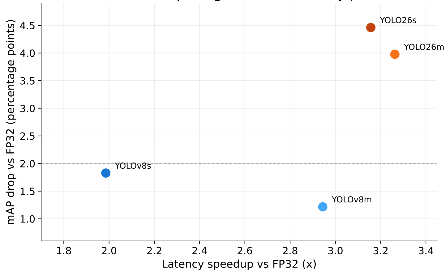
INT8 PTQ: speed gained vs. accuracy paid
