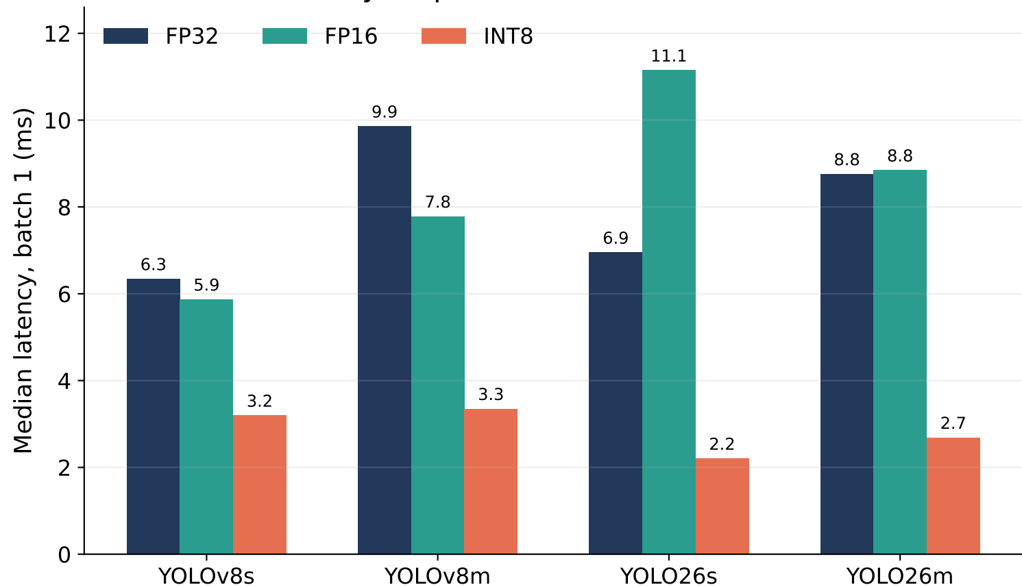
YOLO latency response to FP16 and TensorRT INT8
