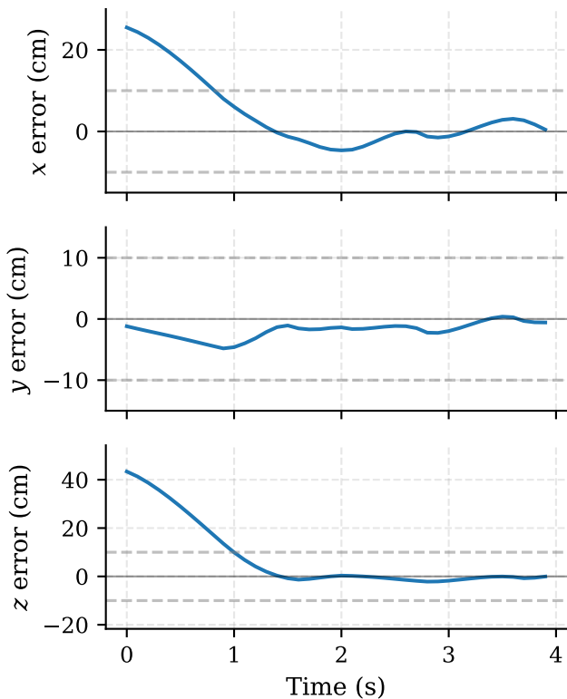
Per-axis position tracking error vs time (traj 13, seed 2)
