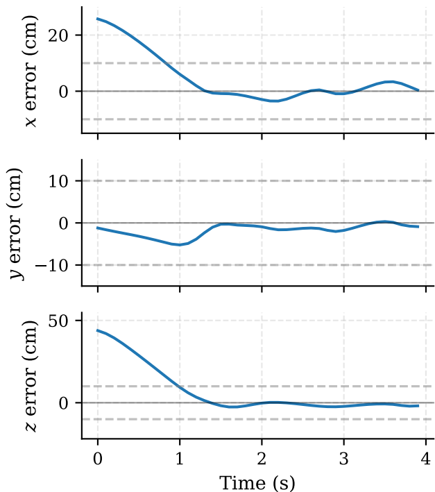
Per-axis position tracking error vs time (traj 13, seed 2)
